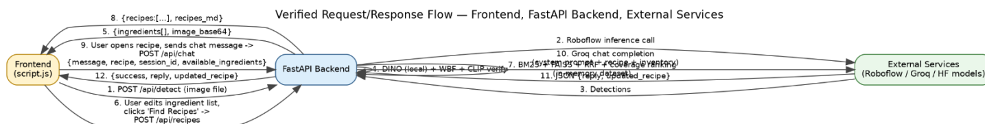
Figure6: Verified request/response interaction flow across the frontend, the FastAPI backend, and the external services it calls for the three main user actions (detect, get recipes, chat)
